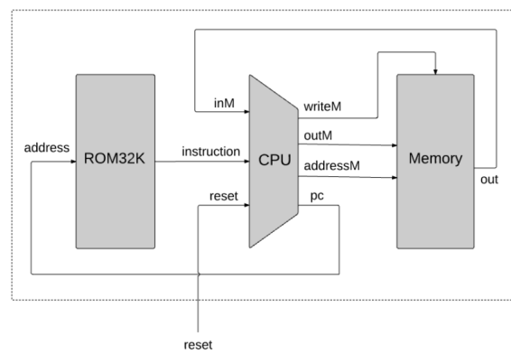
FIGURE 2 – Computer
