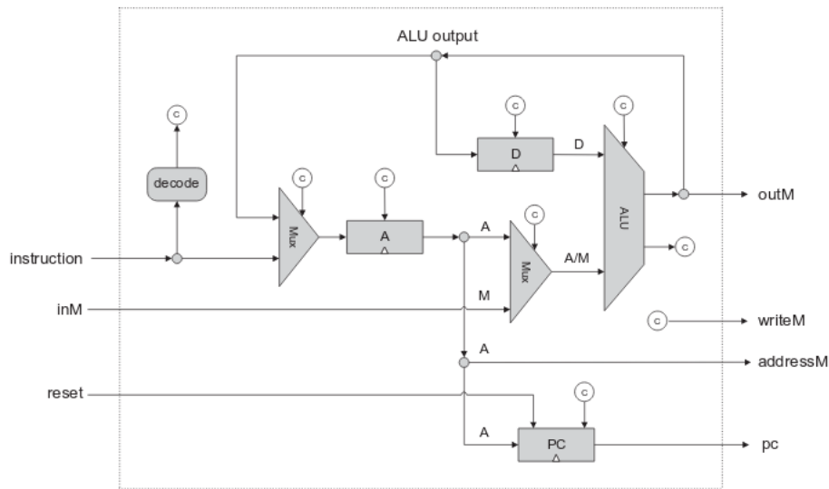
FIGURE 1 – CPU
